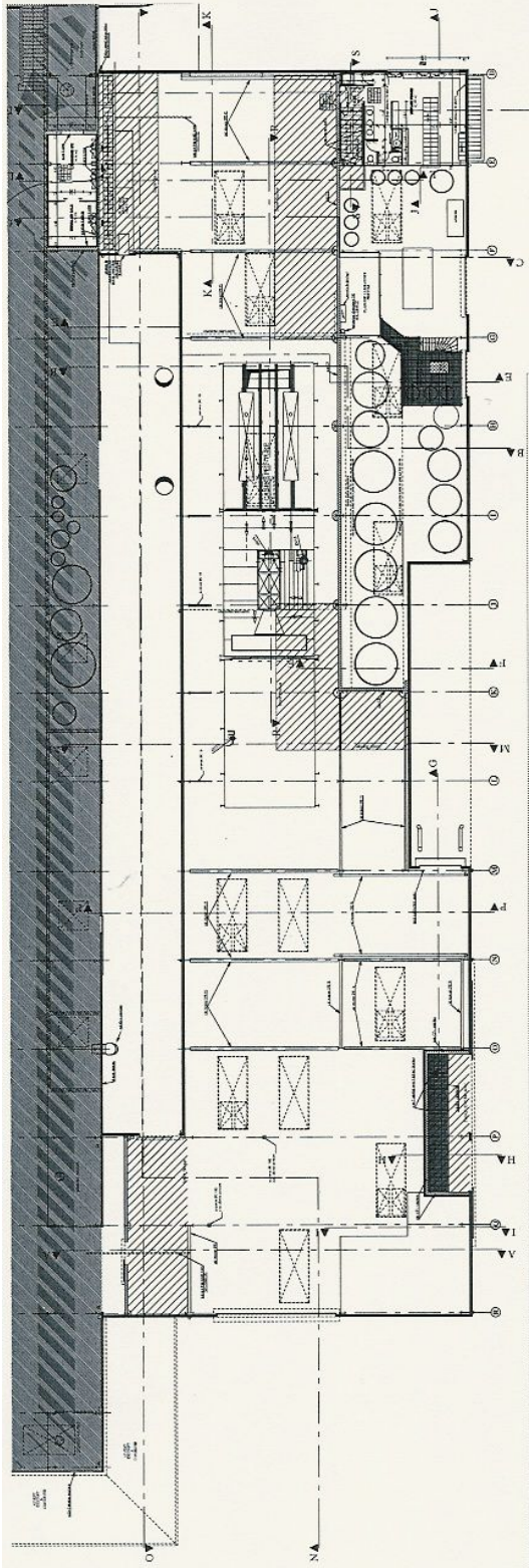
PLAN IER ETAGE
